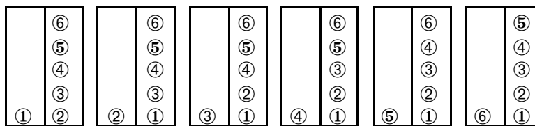
Figure 2.9. There are 6 possible ways to distribute 6 energy units so that the left block has 1 unit and the right block has 5.
