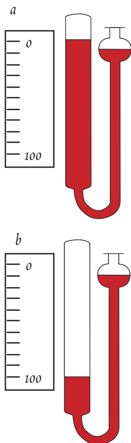
Figure 2.5. An ideal gas thermometer.
