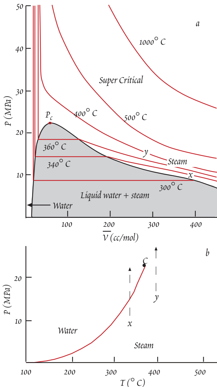
Figure 2.3 (a) Pressure-volume relations for water with isotherm contours. Water and steam coexist only in the shaded area. Both diagrams are examples of phase diagrams, of which we will see a number of other examples. Supercritical fluids exist above P_c . (b) boiling curve for water showing the critical point C, which is at 22 MPa and 373° C. After Nordstrom & Munoz (1986).
