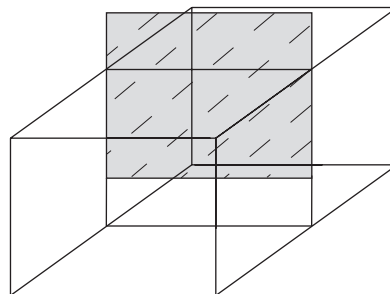
Figure 2.6. A gas-filled box with a removable partition. When the partition is removed, the gases mix. Entropy increases during this process.
