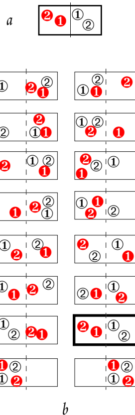
Figure 2.7. Possible distribution of molecules of a red and a black gas in a box before (a) and after (b) removal of a partition separating them.
