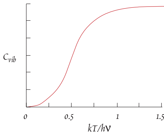
Figure 2.12. Vibrational contribution to heat capacity as a function of kT/h\nu .
