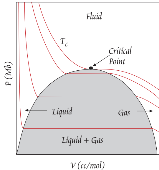
Figure 2.4. Schematic phase diagram of a gas showing two-phase region (shaded) and isotherms. From Nordstrom & Munoz (1986).
