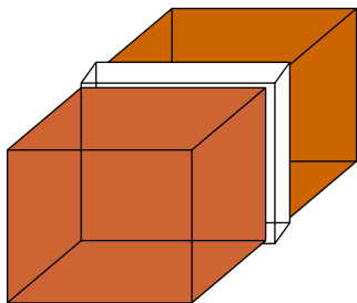
Figure 2.8. Two copper blocks at different temperatures separated by an insulator. When the insulator is removed and the blocks brought in contact, the blocks come to thermal equilibrium. Entropy increases in this process.
