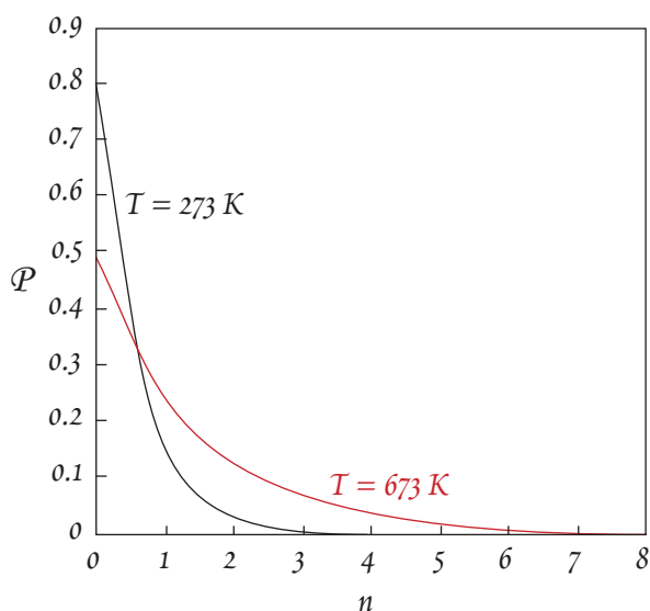
Figure 2.11. Occupation of vibrational energy levels calculated from the Boltzmann distribution. The probability of an energy level associated with the vibrational quantum number n is shown as a function of n for a hypothetical diatomic molecule at 273 K and 673 K.
