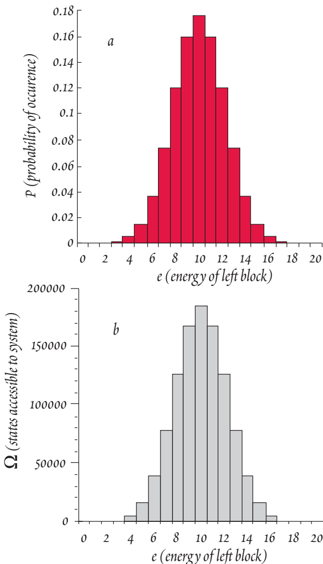
Figure 2.10. (a) Probability of one of two copper blocks of equal mass in thermal equilibrium having e units of energy when the total energy of the two blocks is 20 units. (b) \Omega , number of states available to the system (permutations of energy distribution) as a function of e .
